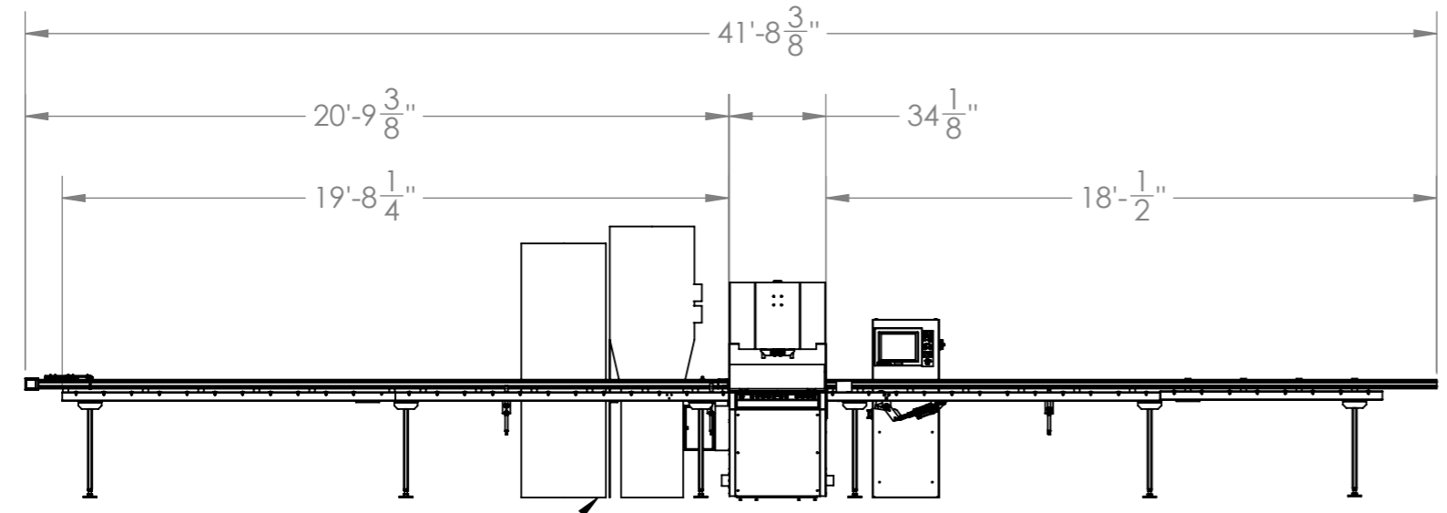
FRONT VIEW SHEET SCALE
